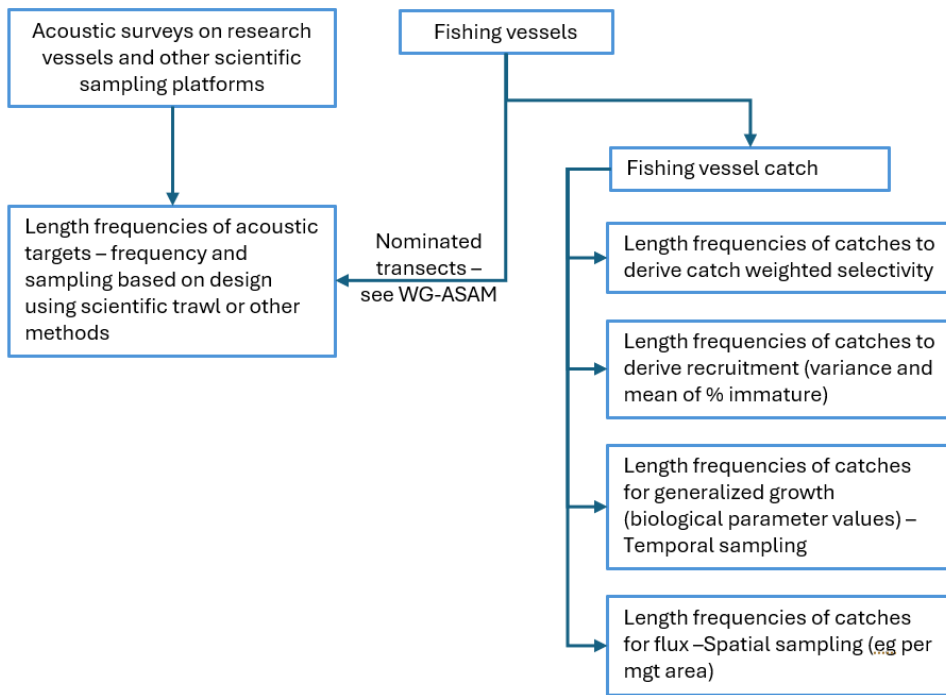
Figure 1: Schematic of key uses of krill length frequency data.
