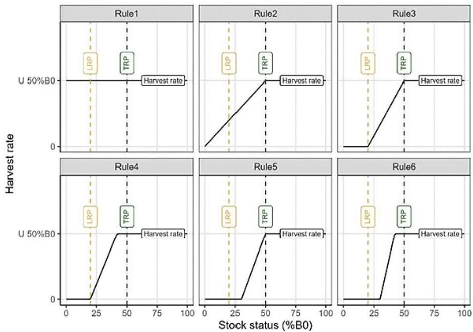
Figure 2: Candidate harvest control rules evaluated for CCAMLR integrated toothfish stock assessments. Black lines indicate the applied harvest rates U given spawning stock status (Stock status (% B_0 )). For example, in Rule 1, the harvest rate is equal to U_{50\%B_0} independent of spawning stock status. In Rule 2, the harvest rate increases linearly from 0 when spawning stock status is also at 0, to U_{50\%B_0} when spawning stock status is at the TRP (dashed green line), and is equal to U_{50\%B_0} when spawning stock status above the TRP. In Rule 3, the harvest rate is 0 for spawning stock status below the LRP (dashed orange line), increases linearly for spawning stock status between the LRP and TRP, and is equal to U_{50\%B_0} when spawning stock status is above the TRP.
