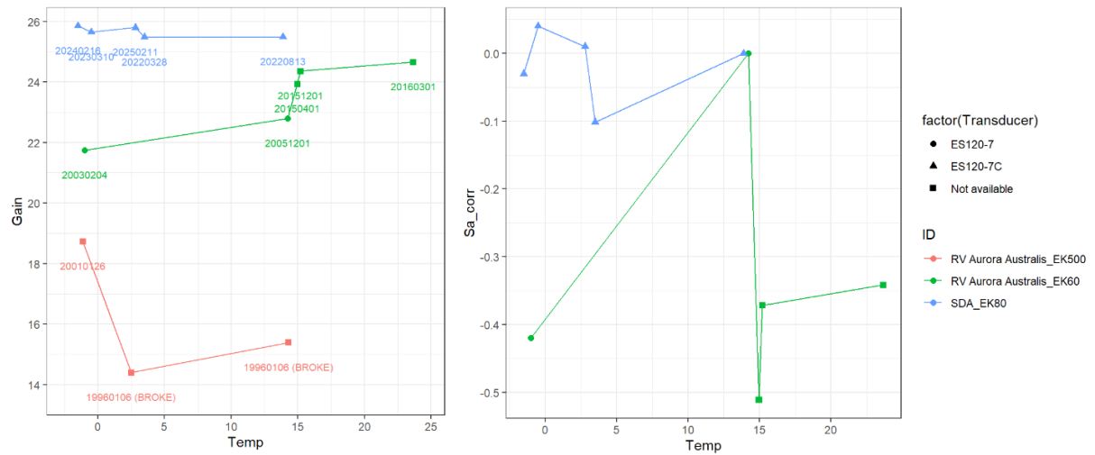
Figure 1: Results of how echosounder Gain (left) and S_a correction (right) vary with temperatures for different platforms and transducers. Labels on the Gain plot are dates of calibration. Note that ice windows on the RV Aurora Australis were changed between 2005 and 2015 and are the likely source of the change at this time.
